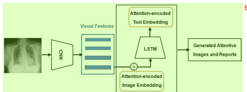
Fig. 6 Attention-based framework for medical report generation 7
