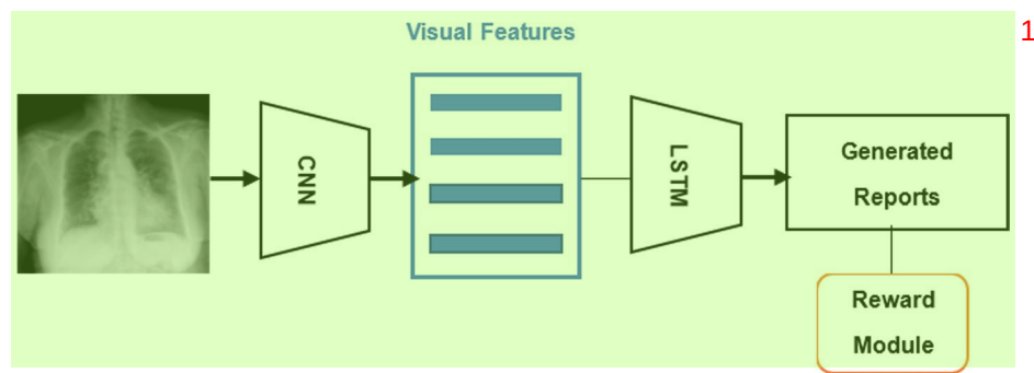
Fig. 7 Reinforcement learning-based framework for medical report generation
